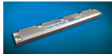
A flat Super Air Knife, only 11/16" thick, blows plastic fibers from a mold used to make integrated circuit chips.
