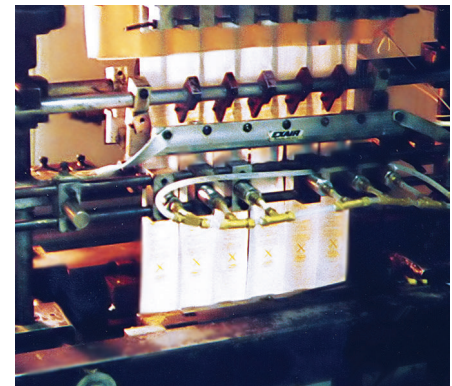
A Model 1212 12" (305mm) Standard Air Knife opens mustard packets prior to fill.
