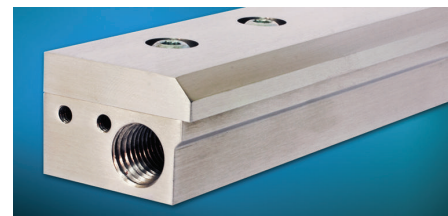
Stainless steel Super Air Knife modified to include extra mounting holes.
